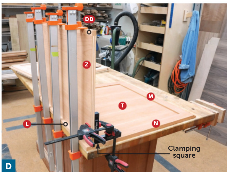
Glue a top panel, with the edging up, into the groove of a back panel. Use a clamping square to keep the panels perpendicular. Clamping to the workbench keeps everything stable.
