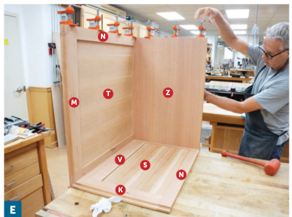
Place a side assembly inside face up on a corner of your bench. Apply glue to the groove and rear rabbet in the side assembly, then clamp the top/back assembly to it.
