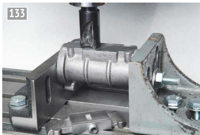
Machining the mating surface for the port face casting.
