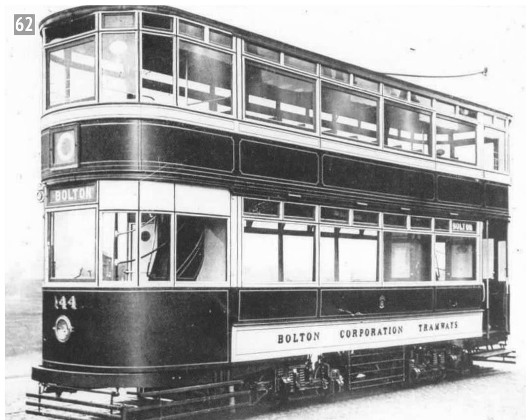
A tram built on a pair of Brill 22E trucks.
