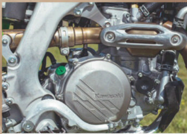
Finger-followers provide high rev limit
