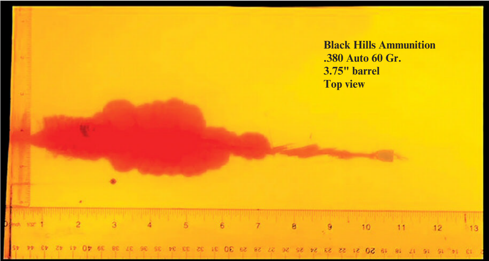
A look at the Black Hills' 60-grain HoneyBadger's performance when fired into properly calibrated 10% gelatin.
