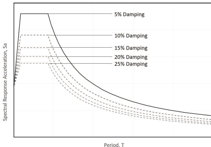
Fig. 1. Example ASCE 7 response spectrum with varying levels of damping.
