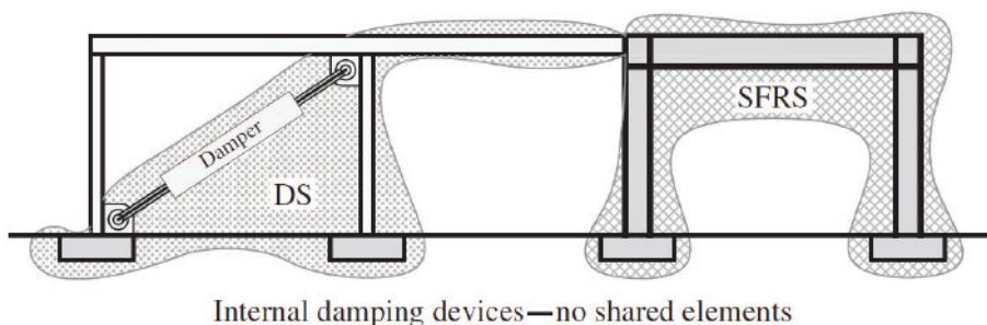
Fig. 2. Steel special moment frame with supplemental damping system.
